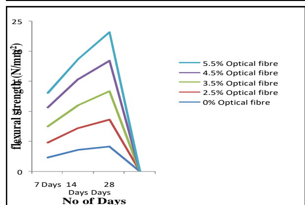
Fig 10: Graph of flexural test of concrete
