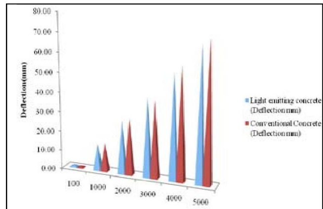
Fig 12: Graph of ANSYS analysis of conventional and optical fibre concrete and deflection
